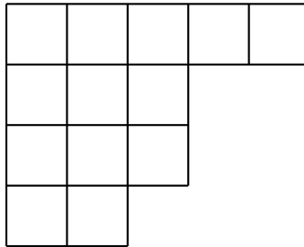
FIGURE 9.3: The partition 4 + 4 + 3 + 1 + 1 .
